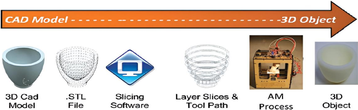
Generalized Additive Manufacturing process Source: Atal Tinkering Lab 7
